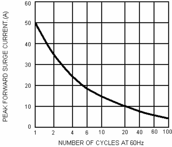
FIG.1-MAXIMUM NONO-REPETITIVE FORWARD SURGE CURRENT PER BRIDGE ELELMENT
